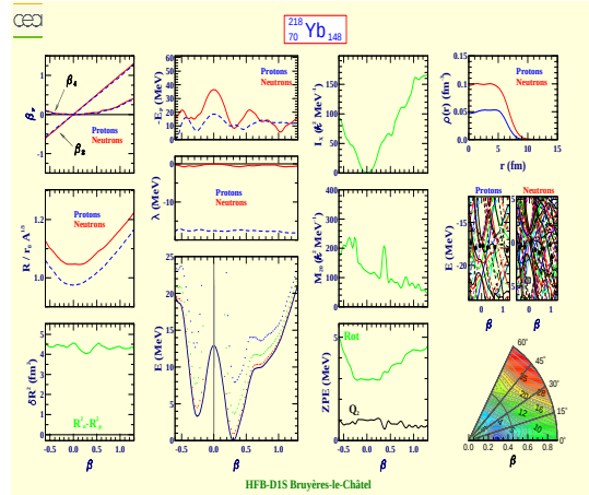
Yterbium 218 (Z=70, N=148)
