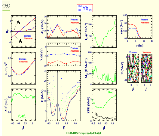
Yterbium 163 (Z=70, N=93)
