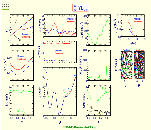
Yterbium 217 (Z=70, N=147)
