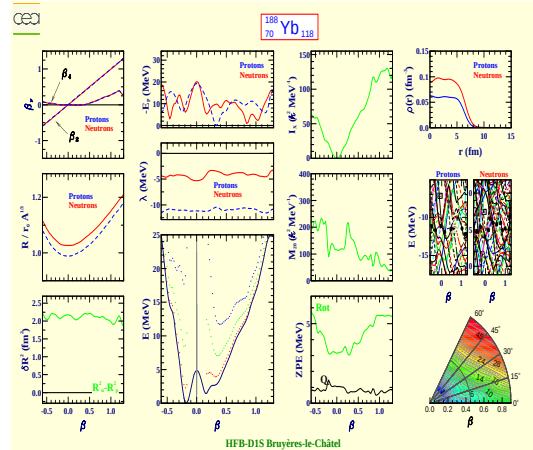
Yterbium 188 (Z=70, N=118)
