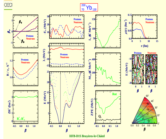
Yterbium 200 (Z=70, N=130)
