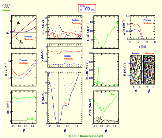
Yterbium 193 (Z=70, N=123)
