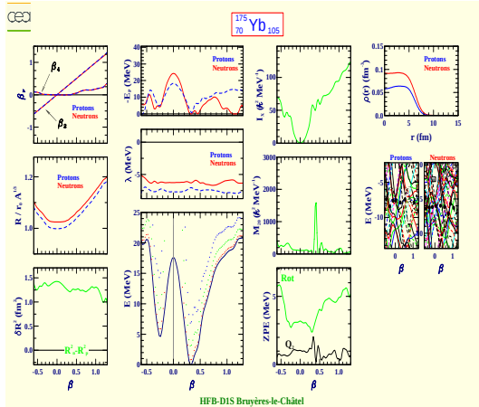
Yterbium 175 (Z=70, N=105)
