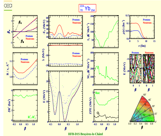
Yterbium 224 (Z=70, N=154)
