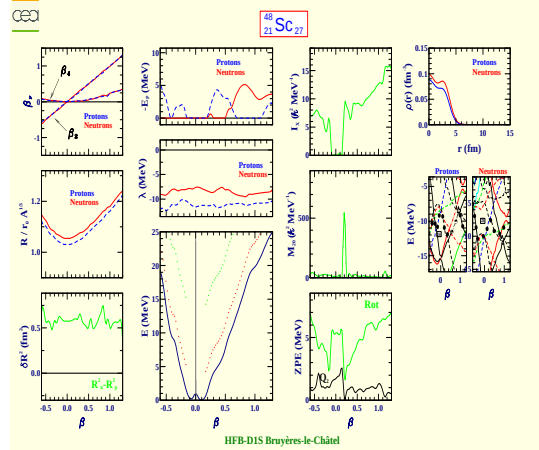
Scandium 48 (Z=21, N=27)
