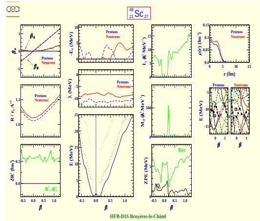
Scandium 48 (Z=21, N=27)
