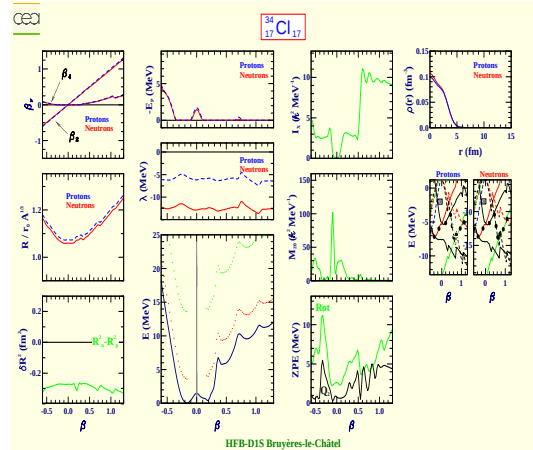
Chlore 34 (Z=17, N=17)
