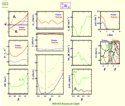
Aluminium 43 (Z=13, N=30)
