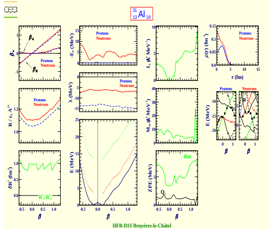
Aluminium 31 (Z=13, N=18)
