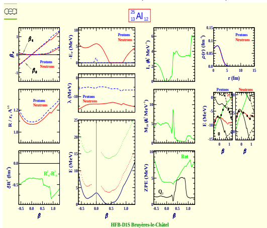
Aluminium 25 (Z=13, N=12)
