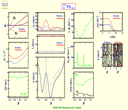
Ytterbium 223 (Z=70, N=153)
