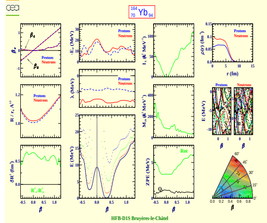
Ytterbium 164 (Z=70, N=94)
