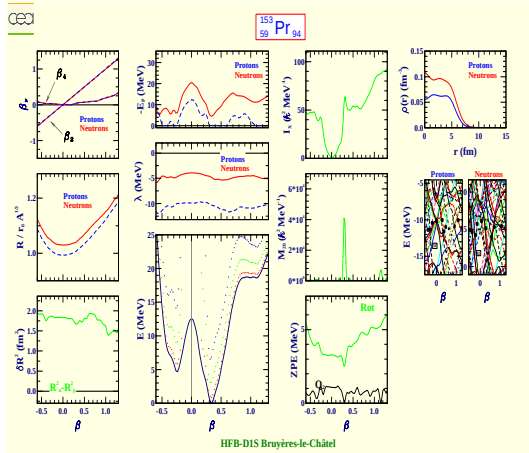
Praseodymium 153 (Z=59, N=94)
