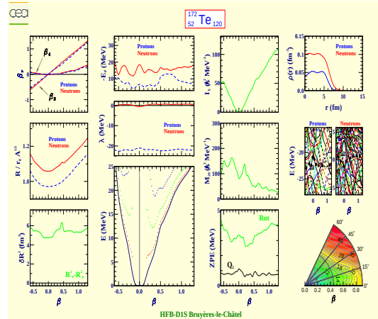
Tellure 172 (Z=52, N=120)
