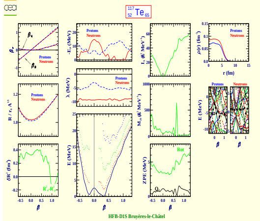
Tellure 117 (Z=52, N=65)
