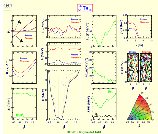
Tellure 142 (Z=52, N=90)
