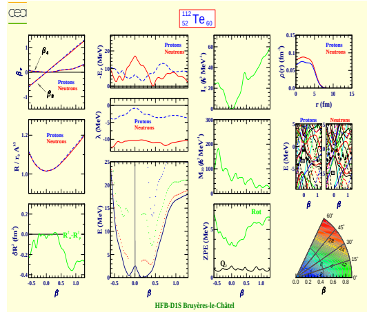
Tellure 112 (Z=52, N=60)
