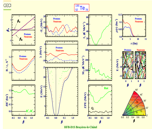
Tellure 130 (Z=52, N=78)
