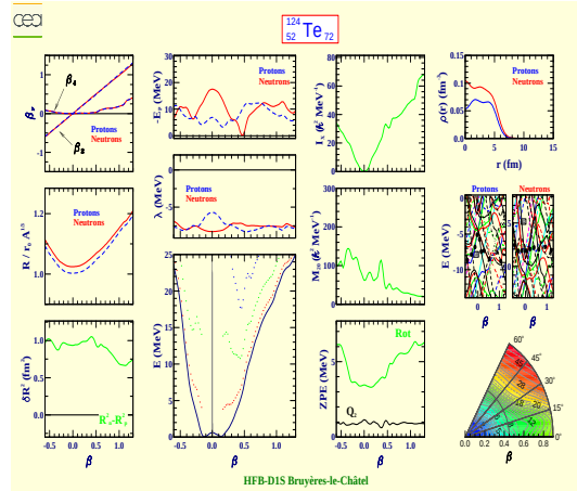
Tellure 124 (Z=52, N=72)
