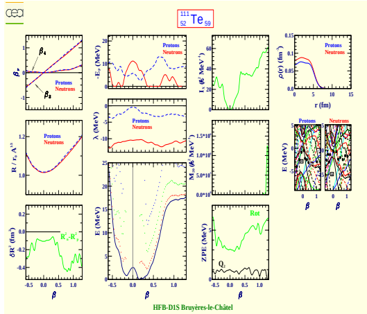
Tellure 111 (Z=52, N=59)
