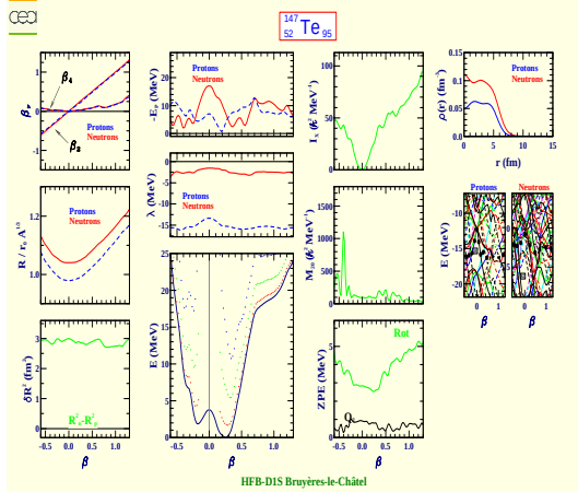
Tellure 147 (Z=52, N=95)
