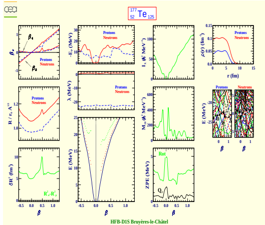
Tellure 177 (Z=52, N=125)
