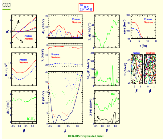
Arsenic 96 (Z=33, N=63)
