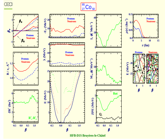
Cobalt 85 (Z=27, N=58)
