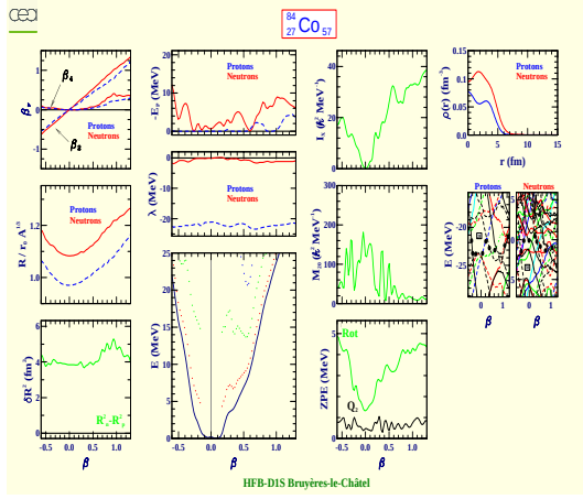
Cobalt 84 (Z=27, N=57)
