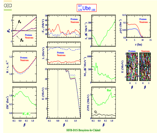
Unbiennium 327 (Z=129, N=198)
