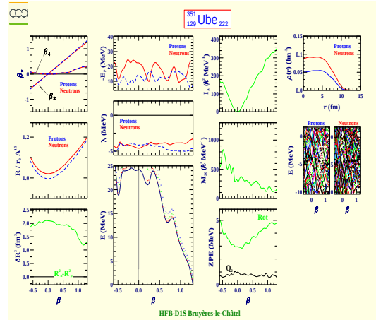
Unbiennium 351 (Z=129, N=222)
