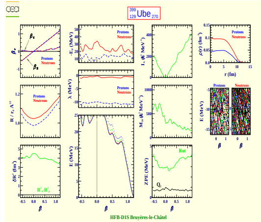
Unbiennium 399 (Z=129, N=270)
