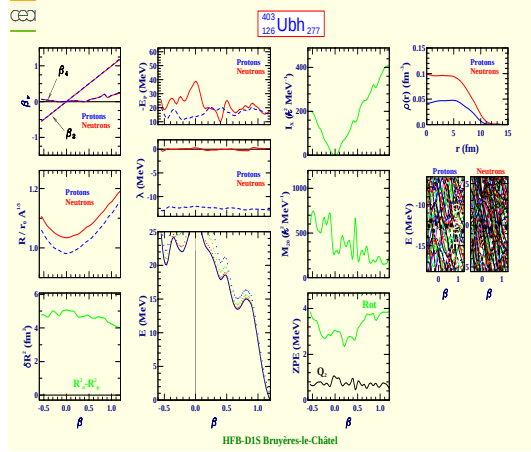
Unbihexium 403 (Z=126, N=277)
