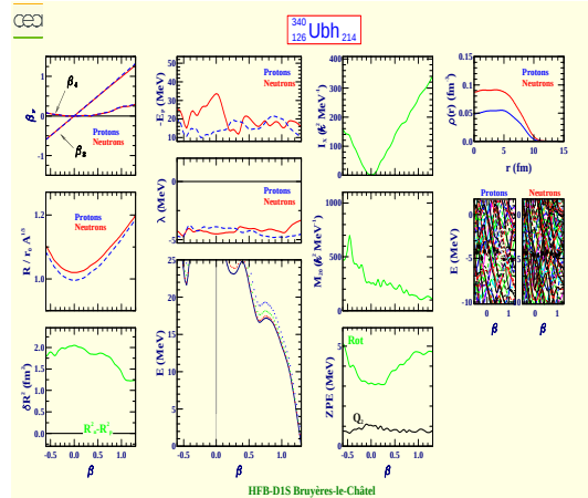
Unbihexium 340 (Z=126, N=214)
