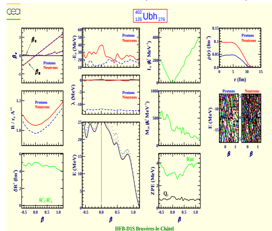
Unbihexium 402 (Z=126, N=276)
