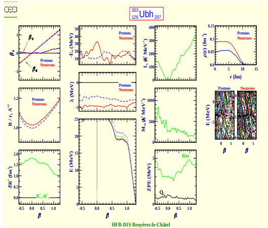
Unbihexium 333 (Z=126, N=207)
