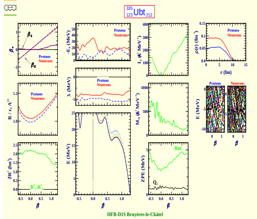
Unbitrium 335 (Z=123, N=212)
