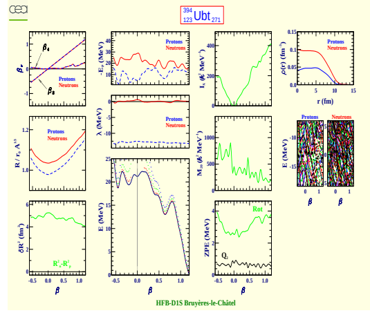
Unbitrium 394 (Z=123, N=271)
