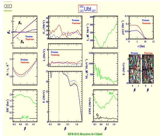
Unbitrium 330 (Z=123, N=207)
