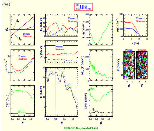
Unbitrium 341 (Z=123, N=218)
