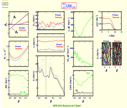
Unbitrium 353 (Z=123, N=230)
