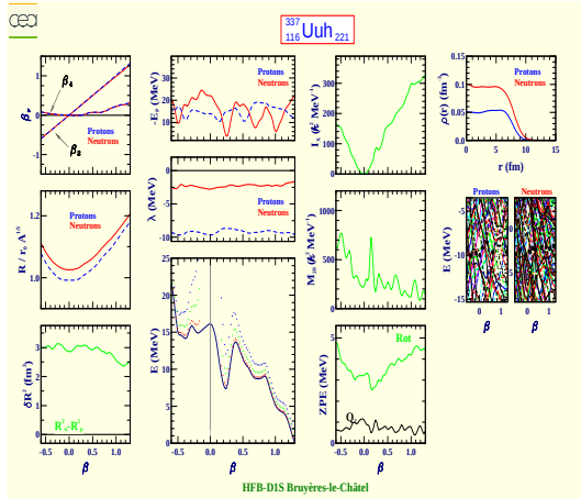
Ununhexium 337 (Z=116, N=221)
